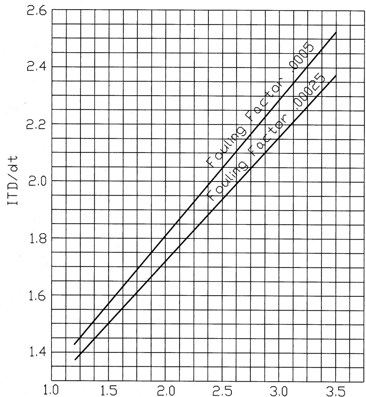
Chart PD-18 - EVP Performance Curve - 20 through 40 Tons
